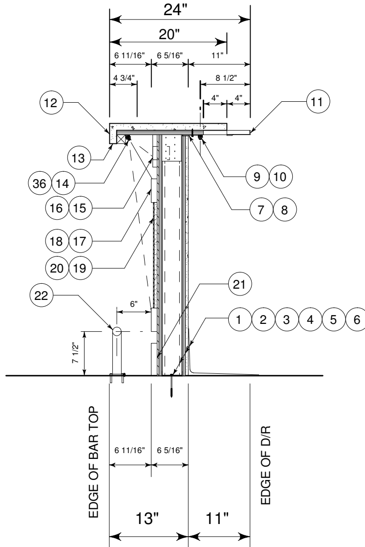
TYPICAL BAR SECTION
